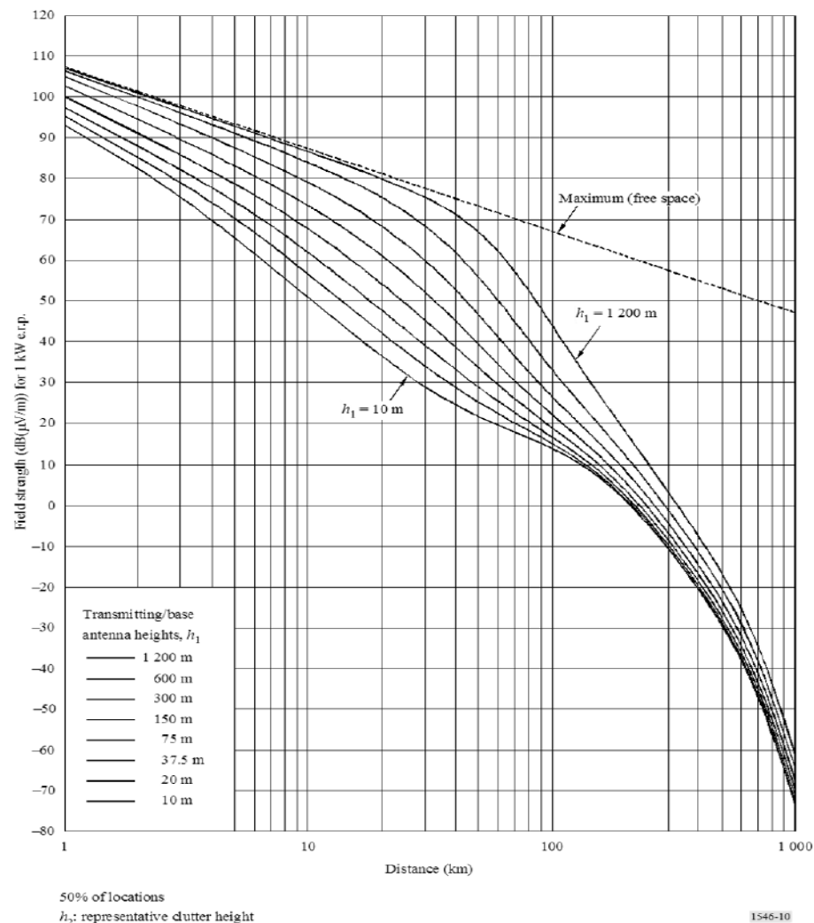
FIGURE 10 600 MHz, land path, 10% time
