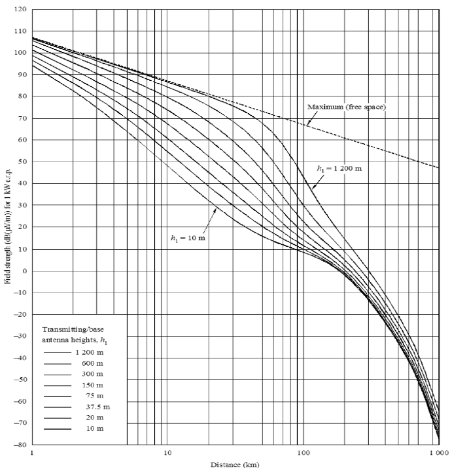
FIGURE 18 2 000 MHz, land path, 10% time
