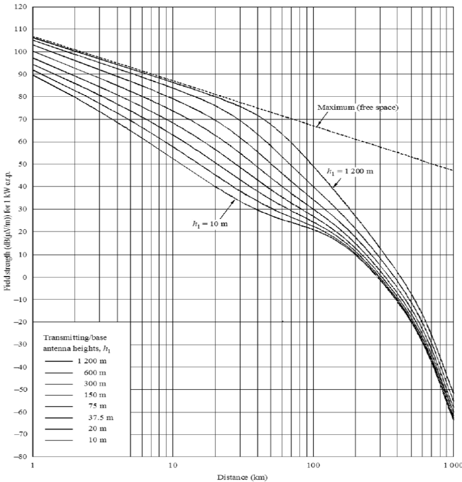
FIGURE 2 100 MHz, land path, 10% time
